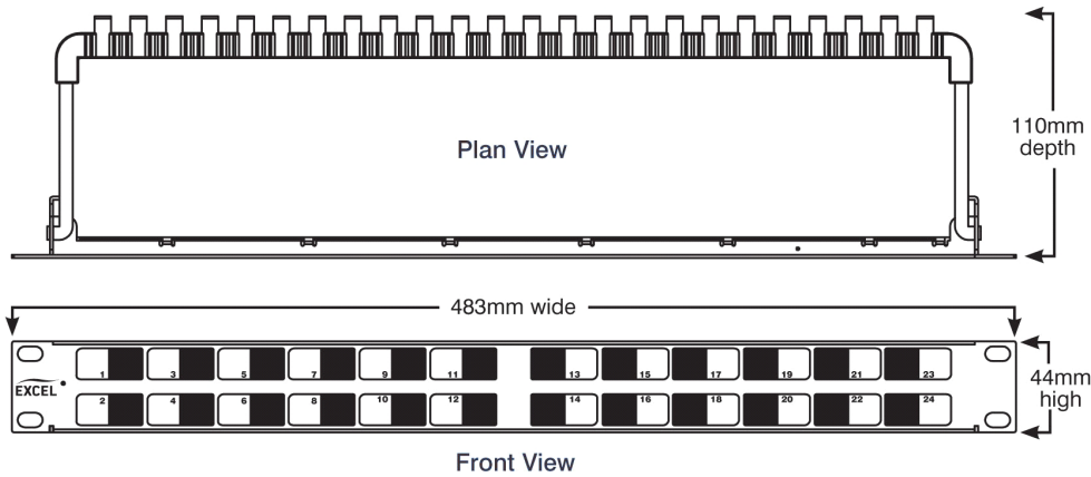
Product drawing
