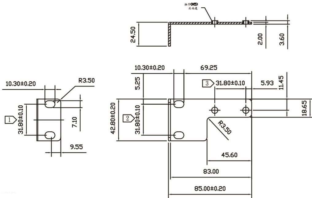
Product drawing (1U version)
