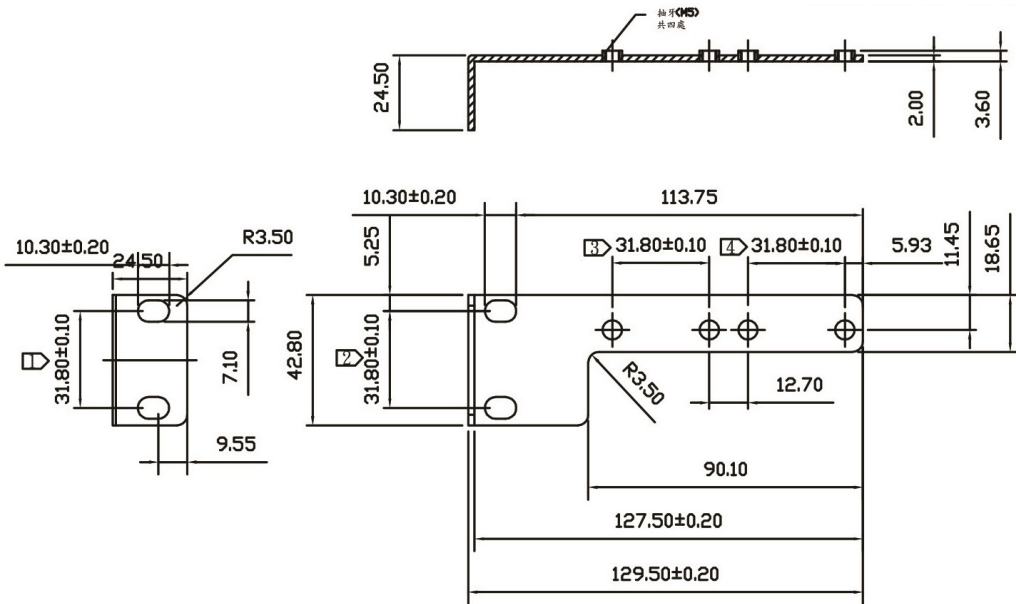
Product drawing (2U version)
