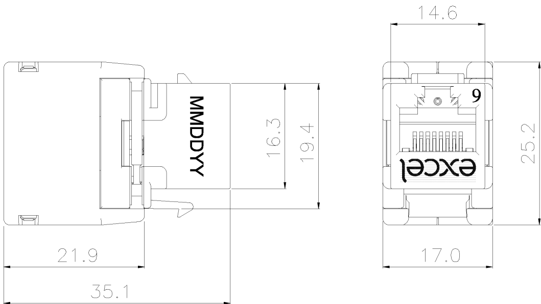
Product drawing
