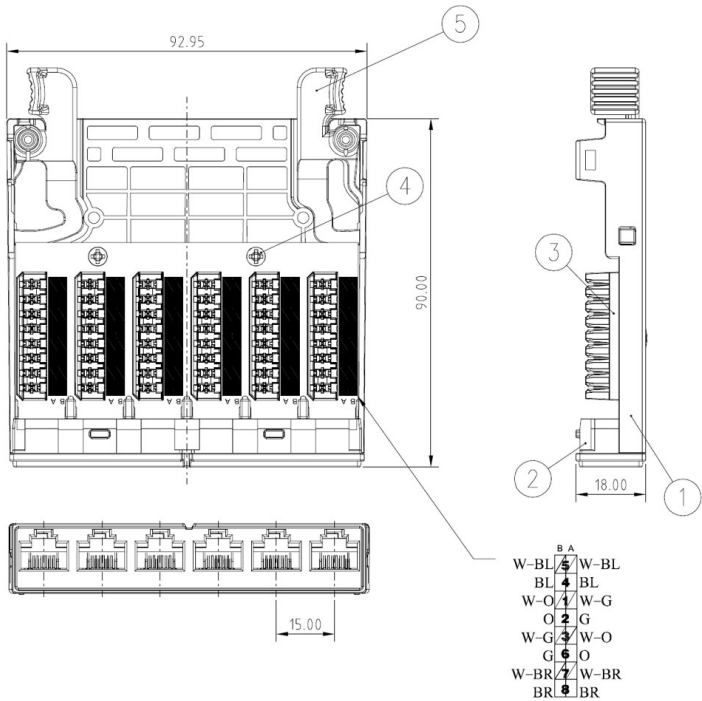
Product drawing
