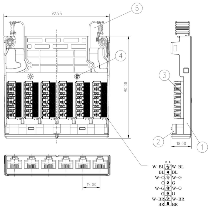
Product drawing
