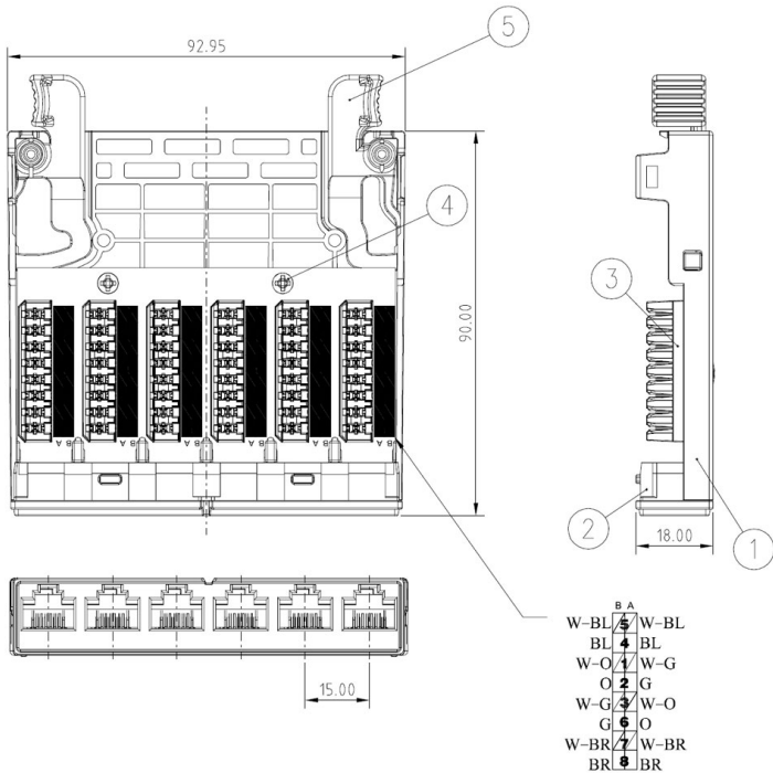
Product drawing
