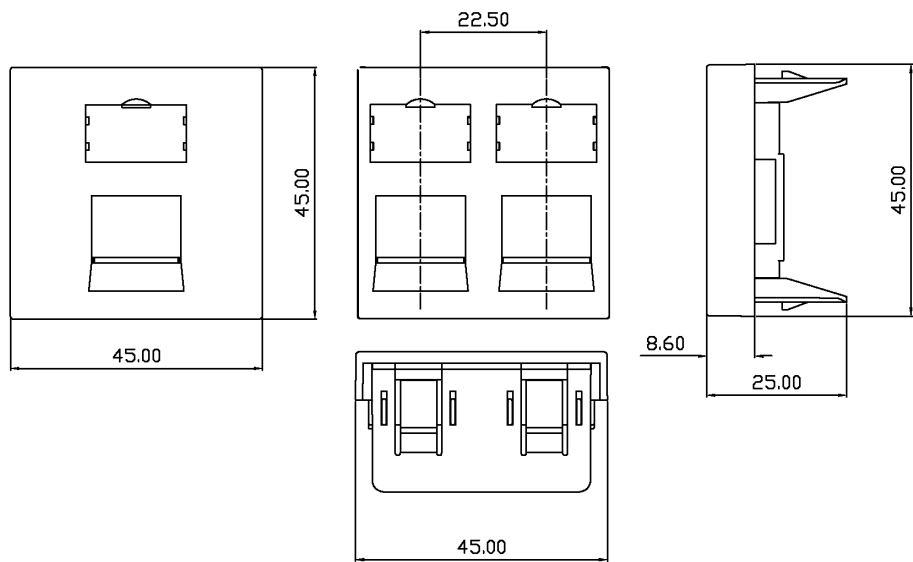
Product drawing
