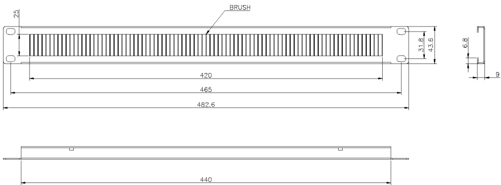
Product drawing (100-599)
