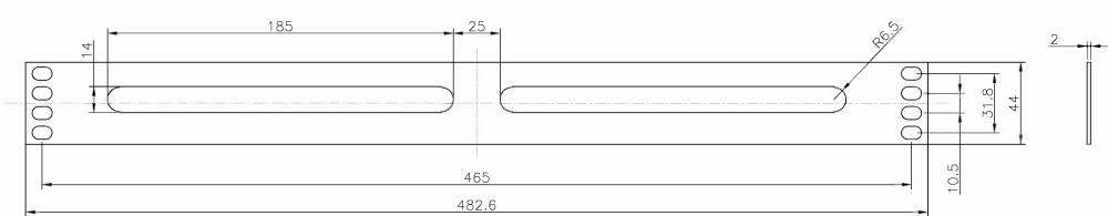
Product drawing (100-610)
