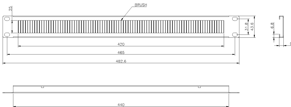
Product drawing (100-599)
