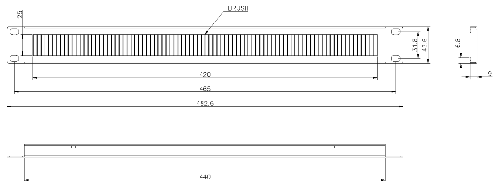
Product drawing (100-599)
