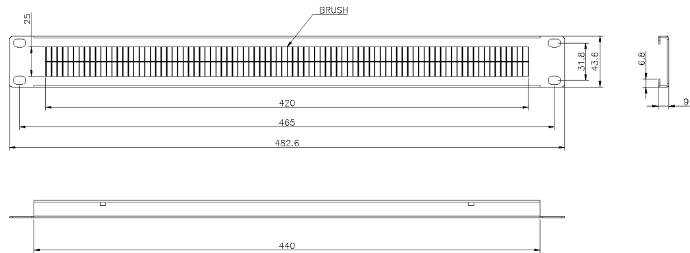
Product drawing (100-595)
