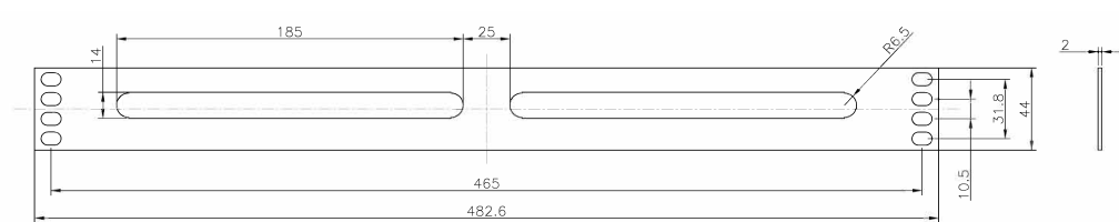
Product drawing (100-610)
