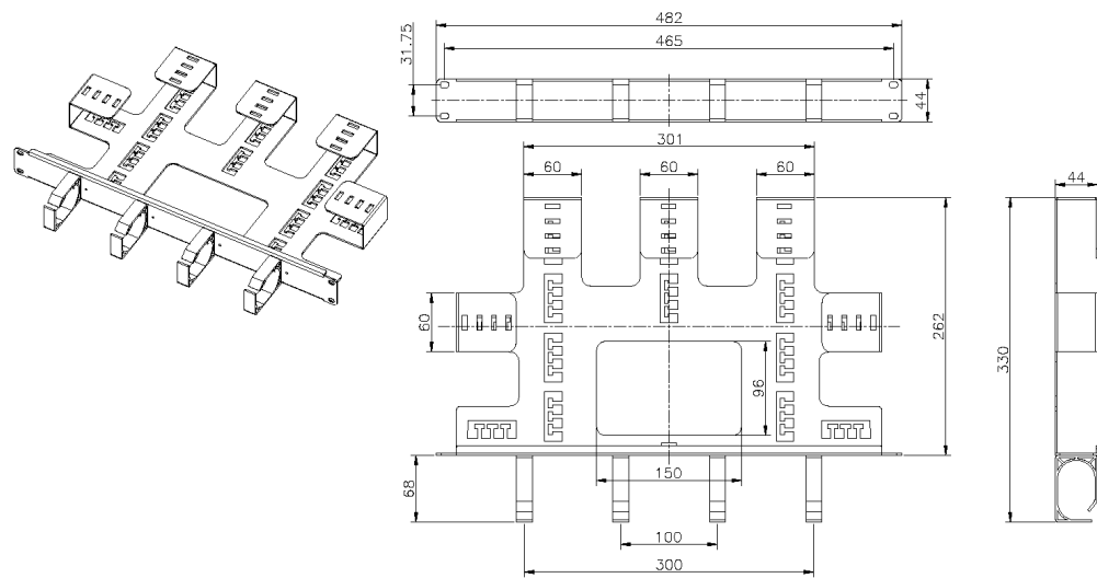
Product drawing
