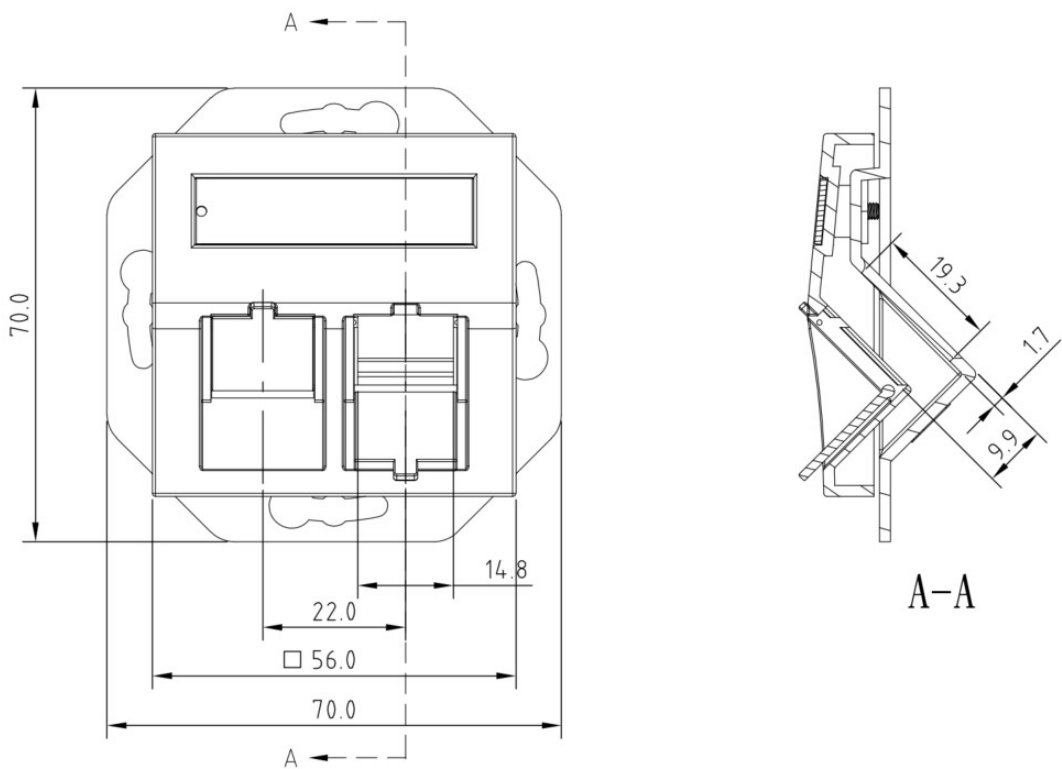
Product drawing
