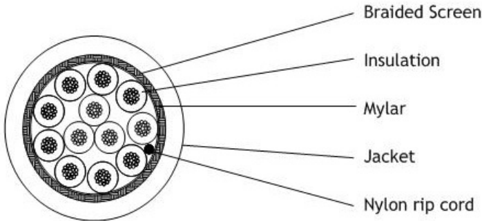
Cross-section diagram
