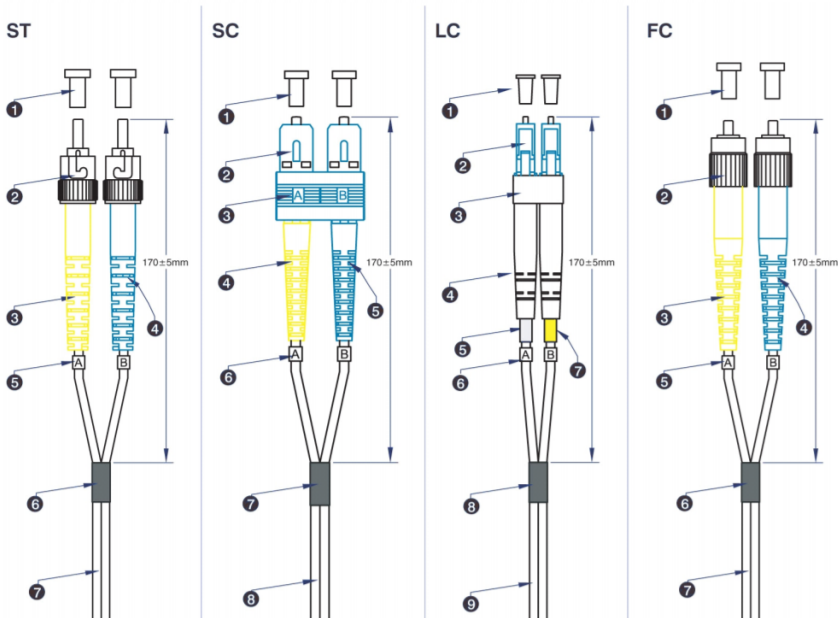
Product drawing
