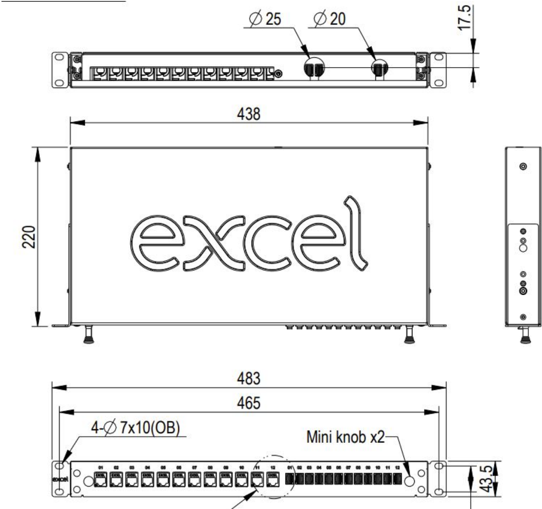
Product drawing
