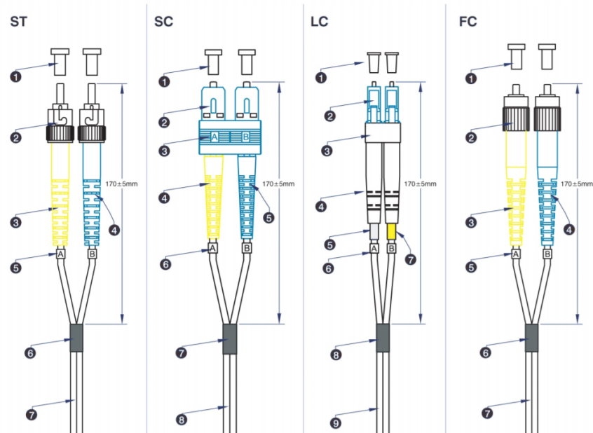
Product drawing
