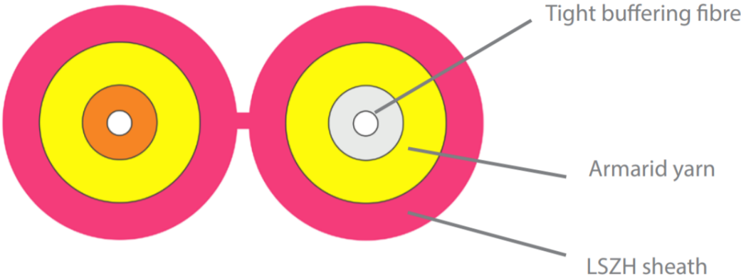
Cross-section diagram
