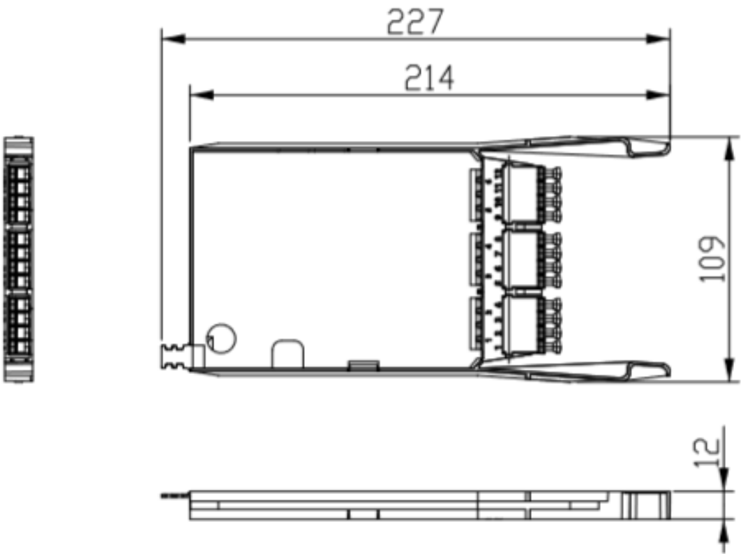
Product drawing
