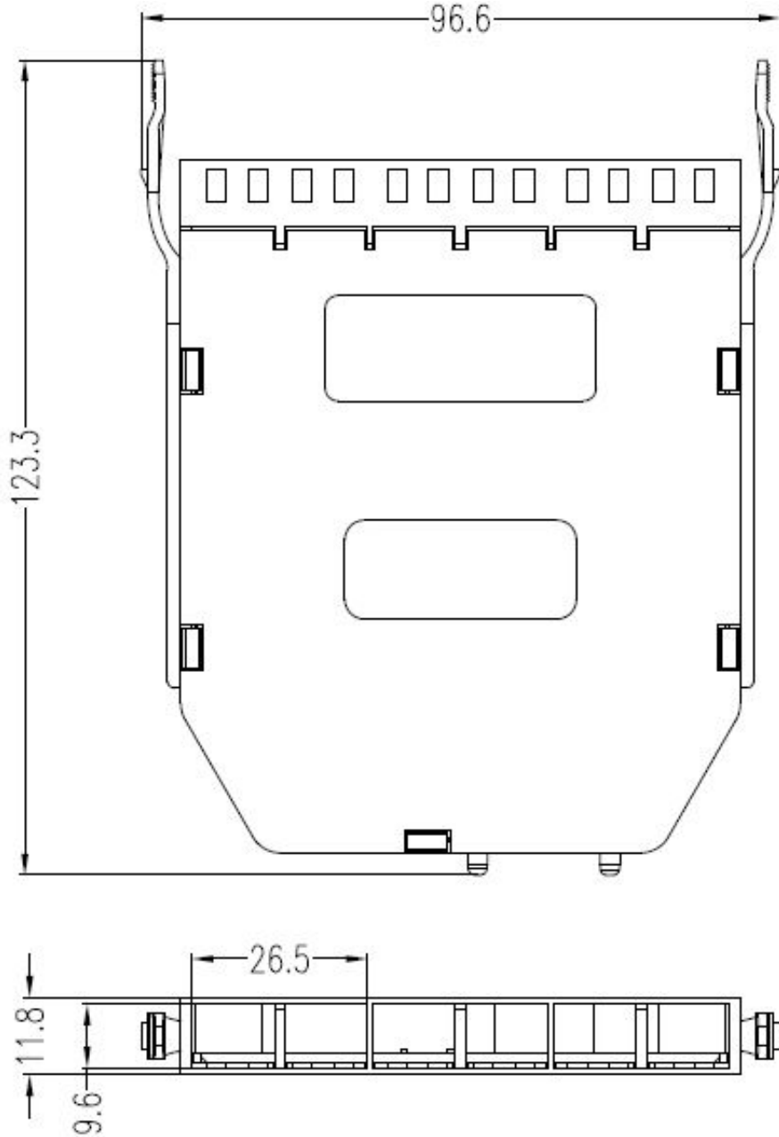
Product drawing
