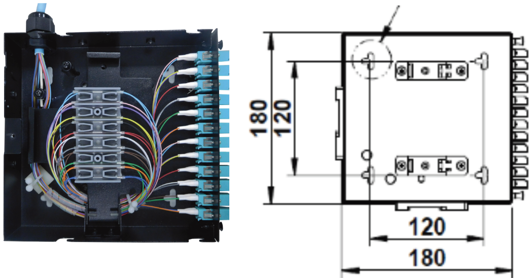
Product drawing
