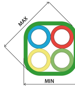
4-Way
