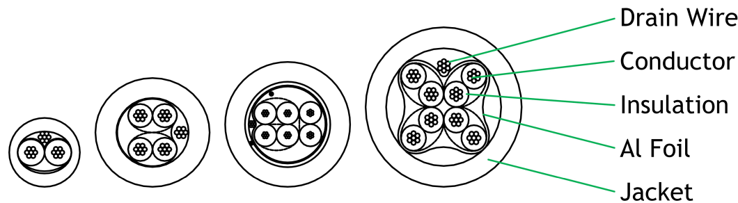
Cross-section diagram
