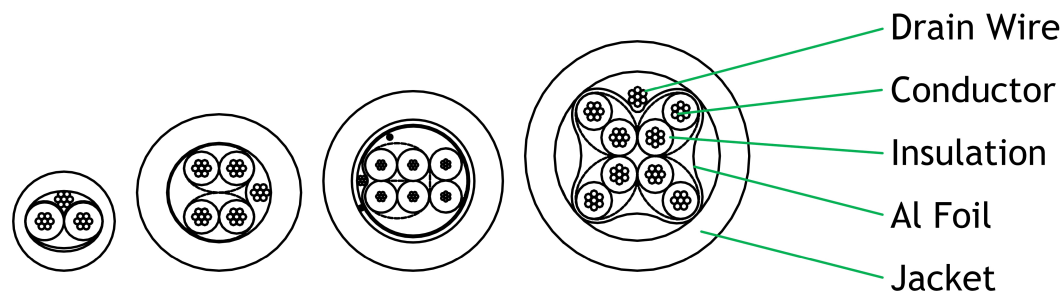
Cross-section diagram
