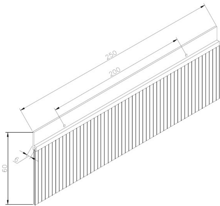
Product drawing
