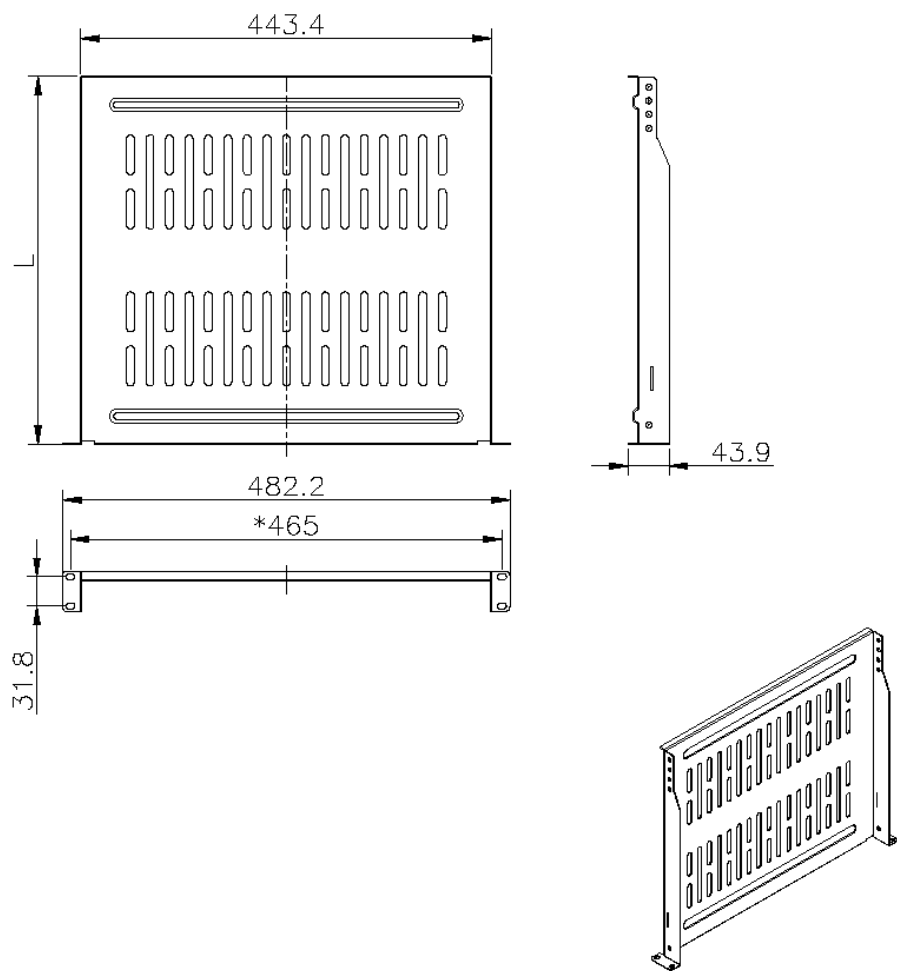
Product drawing
