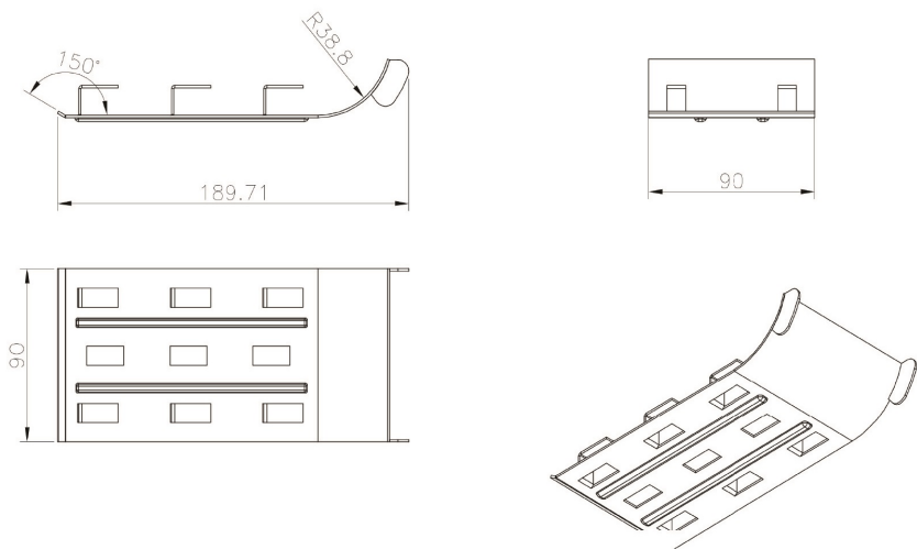
Product drawing (roof bracket)
