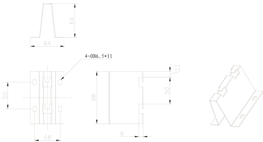
Product drawing (waterfall bracket)
