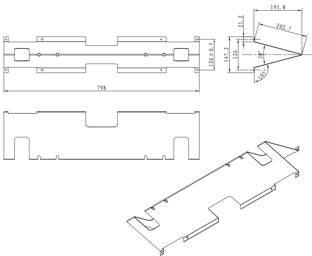
Product drawing
