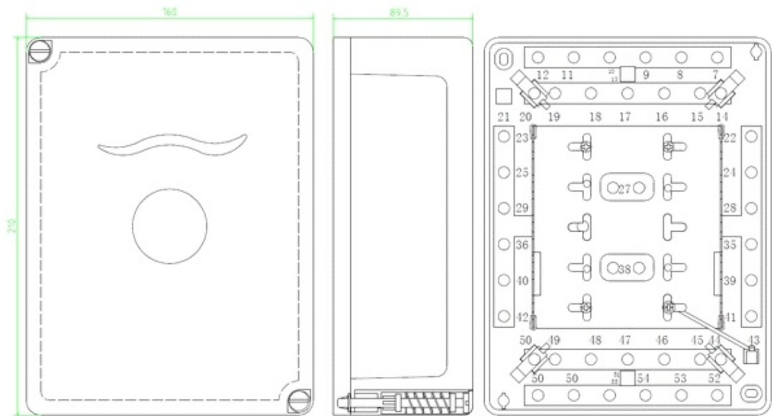
Product drawing
