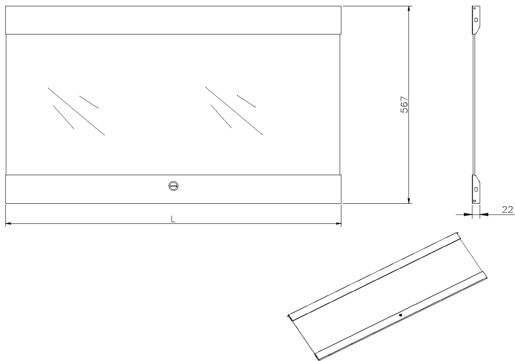
Product drawing
