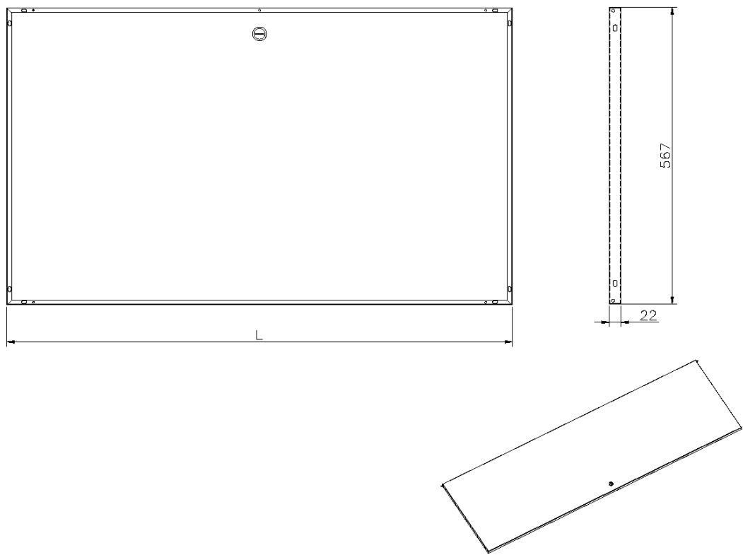
Product drawing
